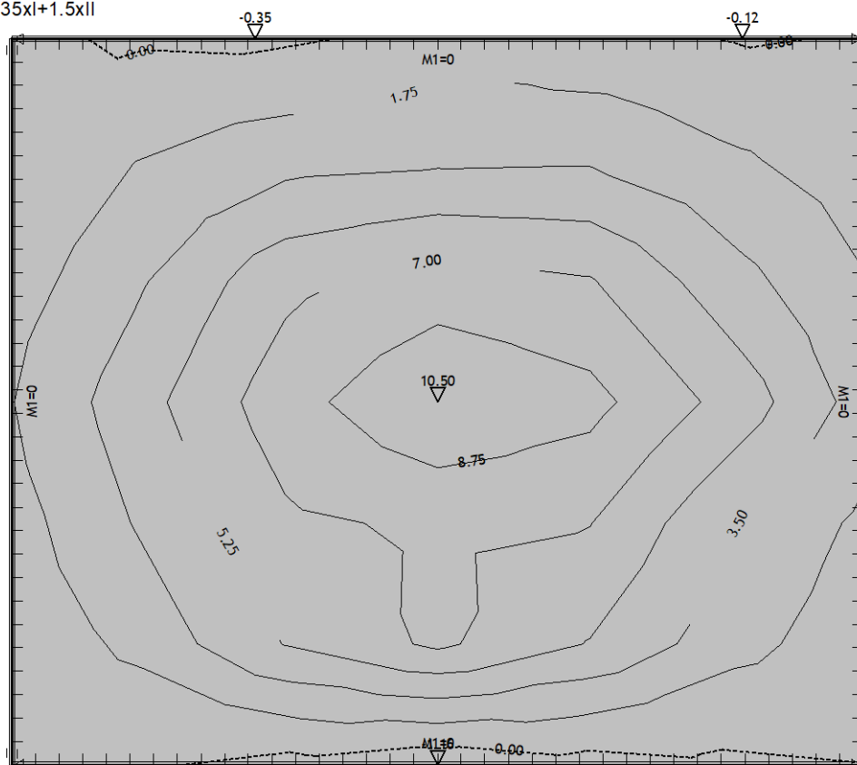
Opt. 5: 1.35xl+1.5xll
